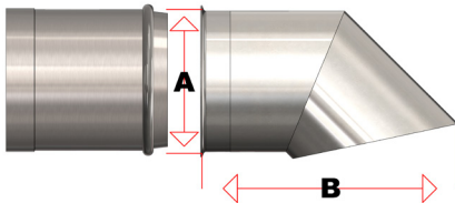
8", 10" & 12" V-BAND STYLE MUFFLER DOWN SPOUTS
